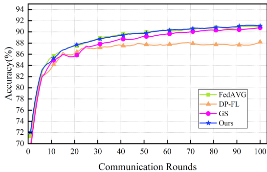
Fig. 7. The test accuracy with respect to communication rounds on Fashion-MNIST dataset, B = 32, E = 3 .
