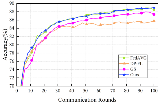
Fig. 10. The test accuracy with respect to communication rounds on FashionMNIST dataset, B = 32 , E = 1 .
