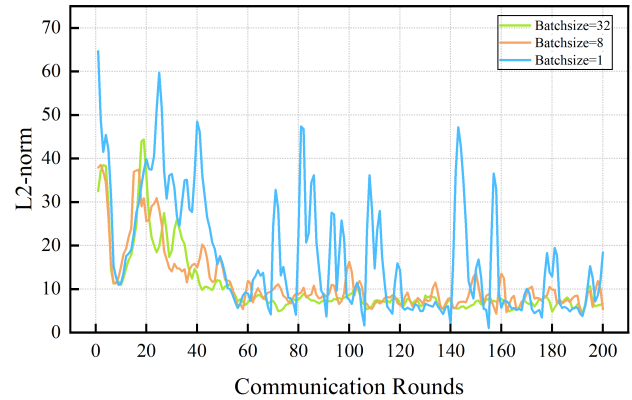
Fig. 4. Gradient norms for different batch sizes.
