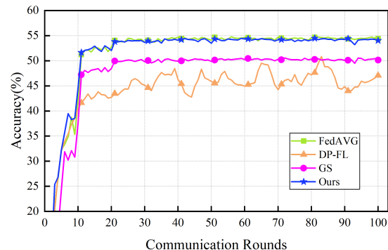
Fig. 9. The test accuracy with respect to communication rounds on Tiny-ImageNet dataset, B = 32, E = 3 .
