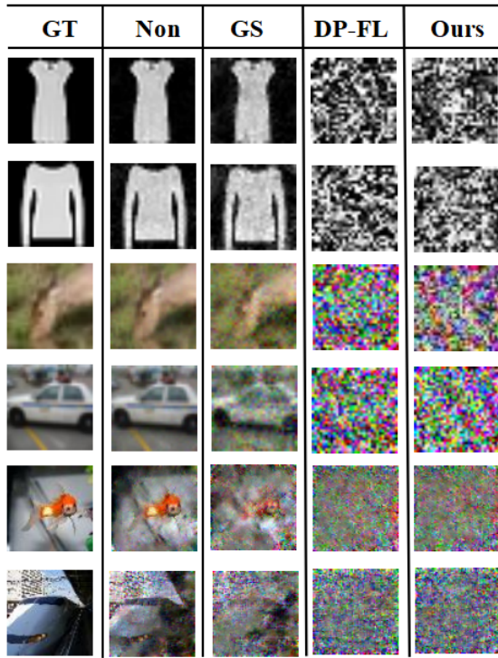
Fig. 5. Resistance of different defense mechanisms, with B = 1 , E = 1 .
